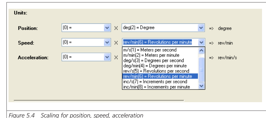
Figure 5.4 Scaling for position, speed, acceleration
