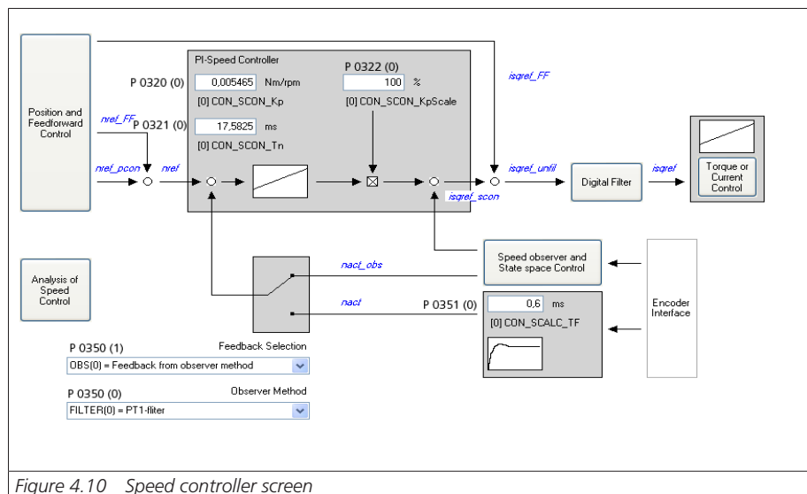
Figure 4.10 Speed controller screen
