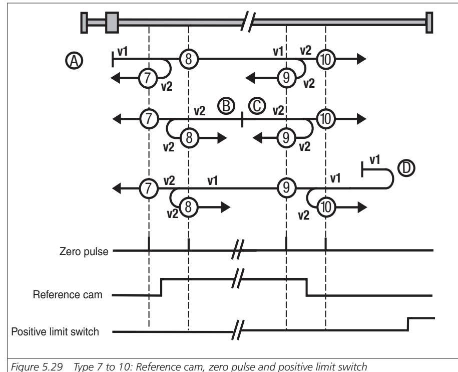
Figure 5.29 Type 7 to 10: Reference cam, zero pulse and positive limit switch
