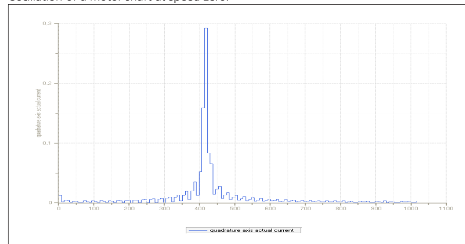
Figure 4.19 Oscillation of a motor shaft under current at standstill without filter
