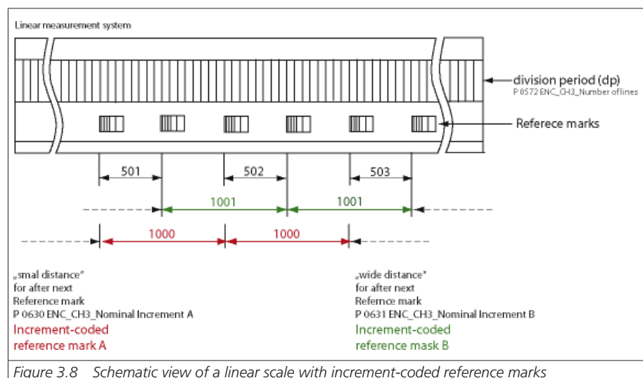
Figure 3.8 Schematic view of a linear scale with increment-coded reference marks
