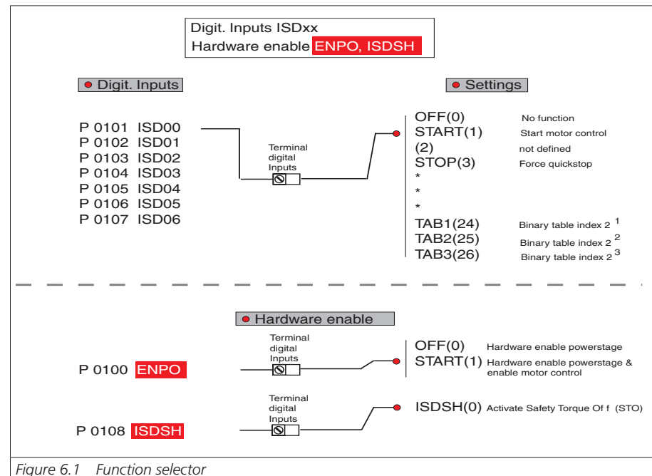
Figure 6.1 Function selector
