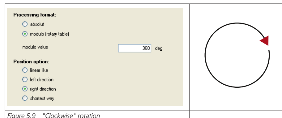
Figure 5.9 "Clockwise" rotation
