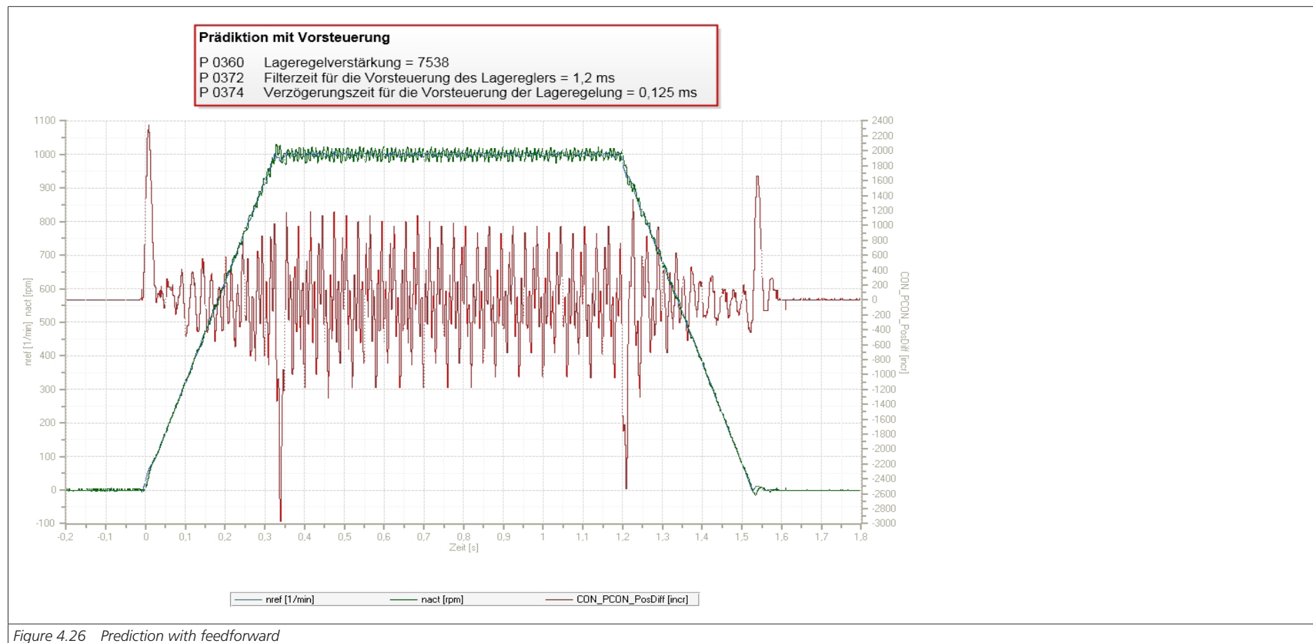
Figure 4.26 Prediction with feedforward
