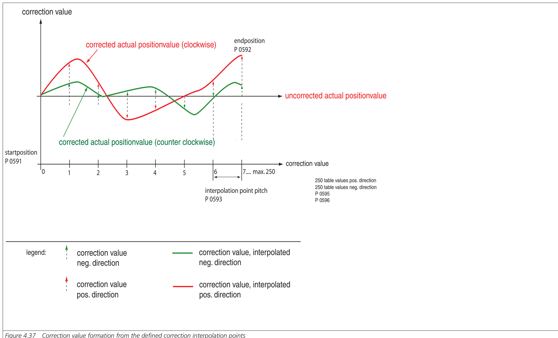
Figure 4.37 Correction value formation from the defined correction interpolation points
