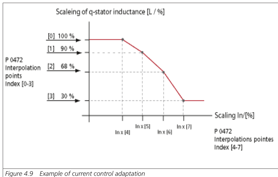
Figure 4.9 Example of current control adaptation
