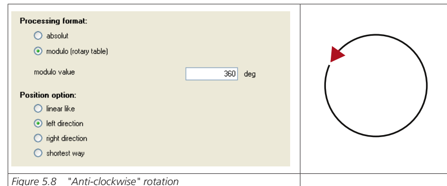
Figure 5.8 "Anti-clockwise" rotation
