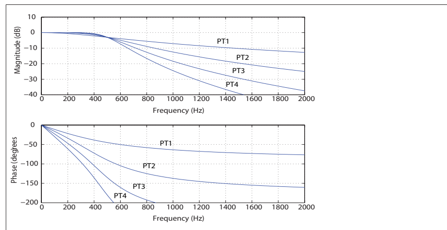
Figure 4.17 Frequency responses of PT1, PT2, PT3, PT4 filters
