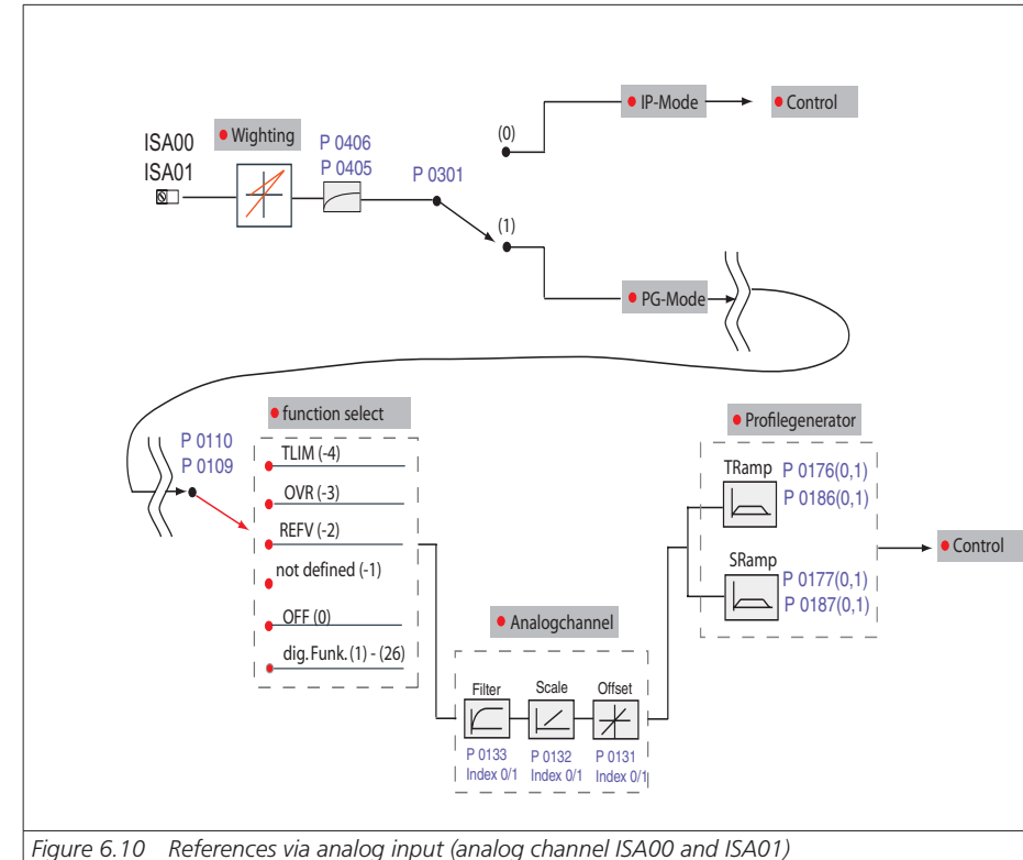
Figure 6.10 References via analog input (analog channel ISA00 and ISA01)
