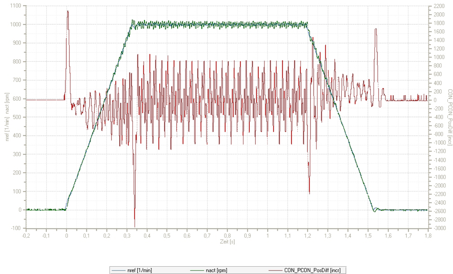
Figure 4.25 Optimized position gain: KP position from 4000 to 7538
