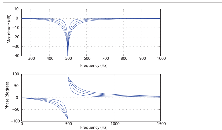
Figure 4.18 Notch filter: Blocking frequency 500 Hz and bandwidths 25, 50, 75 and 100 Hz
