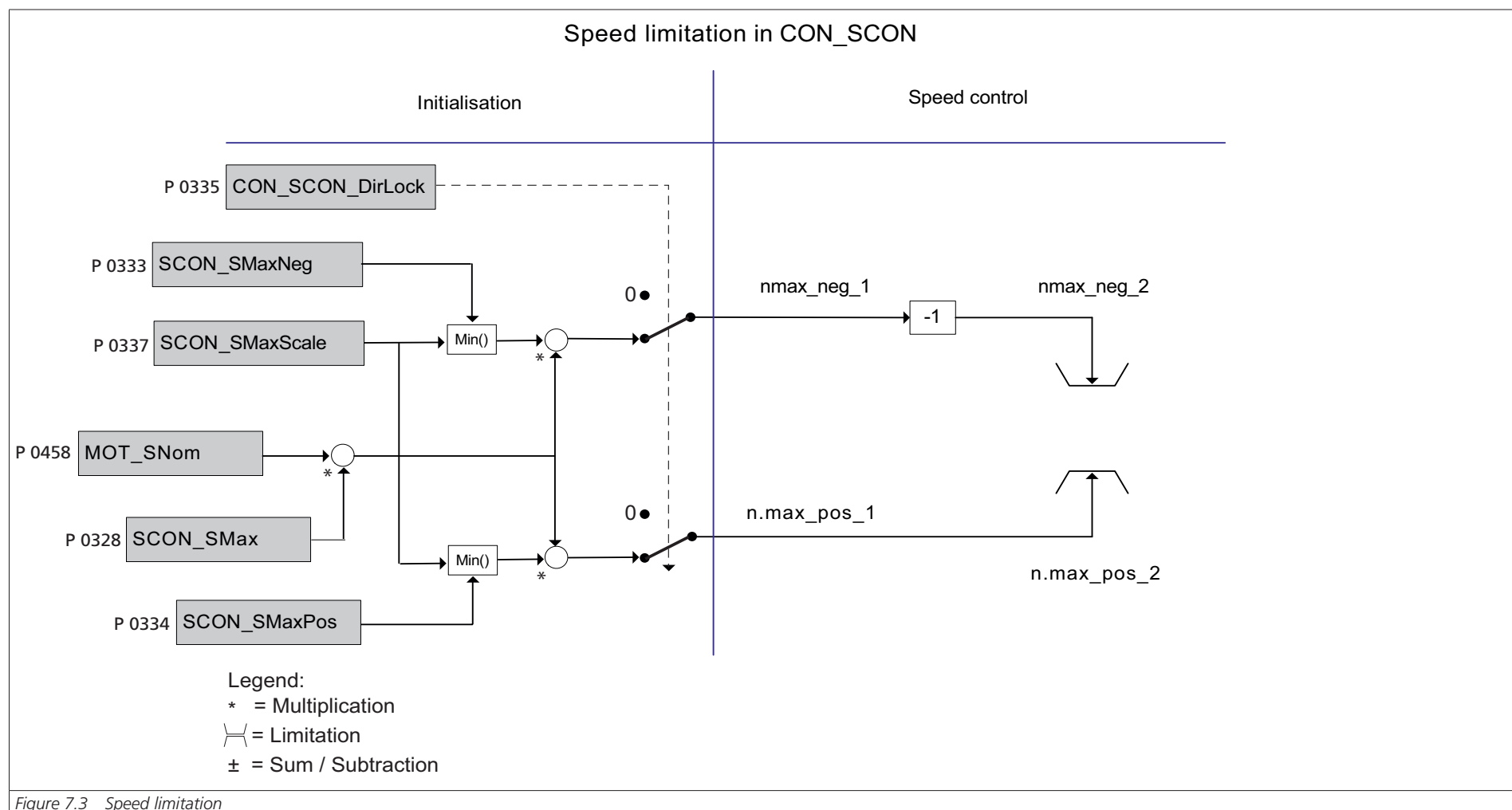
Figure 7.3 Speed limitation
