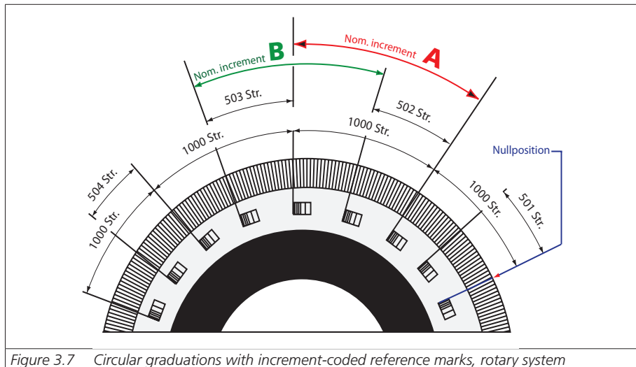
Figure 3.7 Circular graduations with increment-coded reference marks, rotary system
