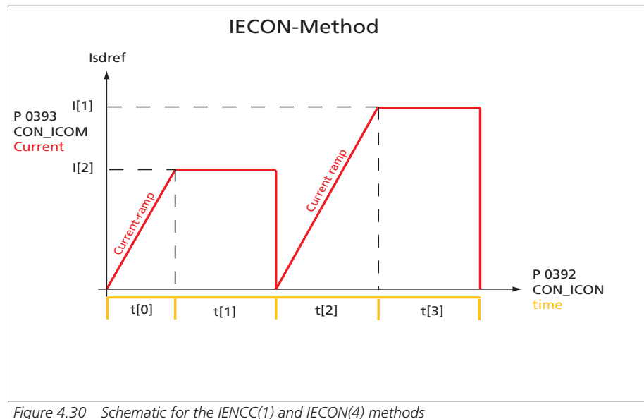
Figure 4.30 Schematic for the IENCC(1) and IECON(4) methods
