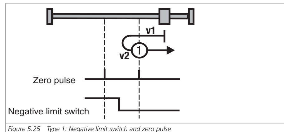
Figure 5.25 Type 1: Negative limit switch and zero pulse
